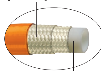
Braided High Tensile Strength Fiber Reinforcement
